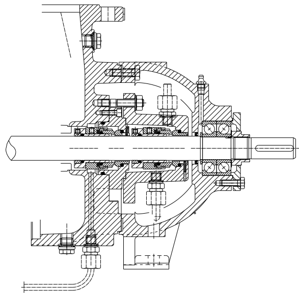
UEA with RBG, (PN40) double mechanicals seal
